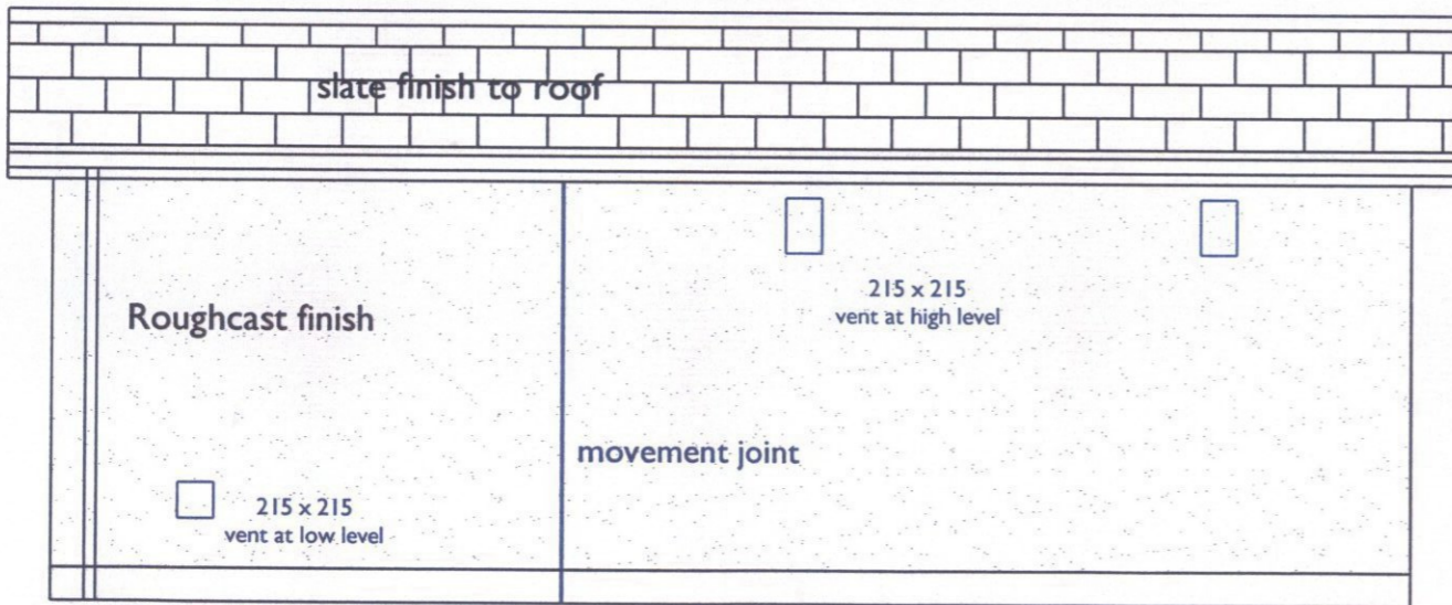
SIDE ELEVATION
