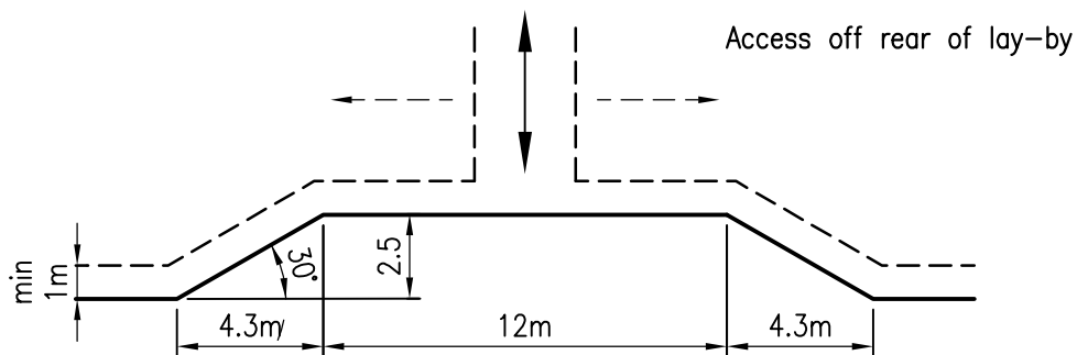
ACCESS LAY-BY FOR 2 DWELLINGHOUSES
