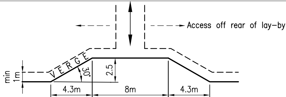
ACCESS LAY-BY FOR A SINGLE DWELLINGHOUSE
