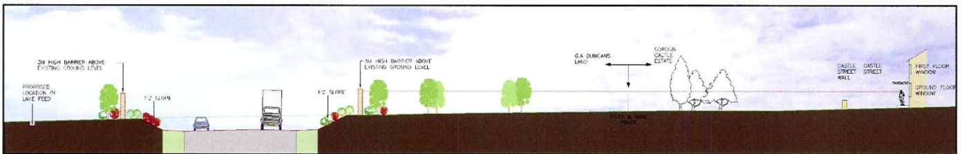
OPTIONS G & H – 3m WALL/BARRIER AT TOP OF CUT SLOPE
