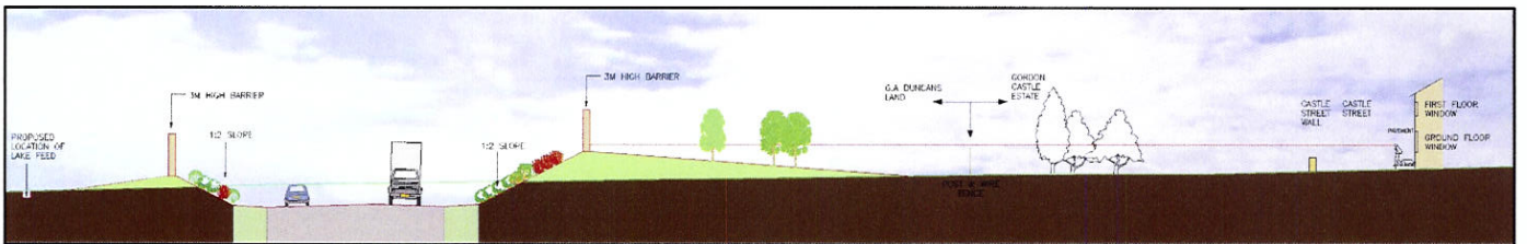
OPTIONS E & F – 3m WALL/BARRIER ON TOP OF FALSE CRESTS
