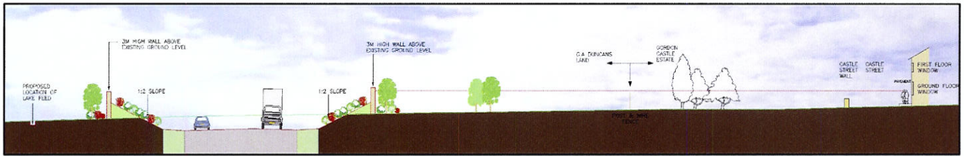
OPTION I – 1:2 SLOPE, 3m WALL, 1m EXPOSED TO CARRIAGEWAY
