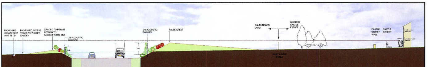
OPTION L - FALSE CREST WITH 1.9m to 3m NOISE BARRIER AT BACK OF VERGE
