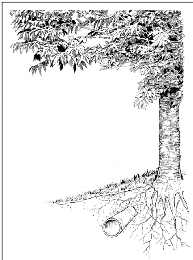
Fig 2: Disruption to roots is minimised by tunnelling utilities under the tree.
